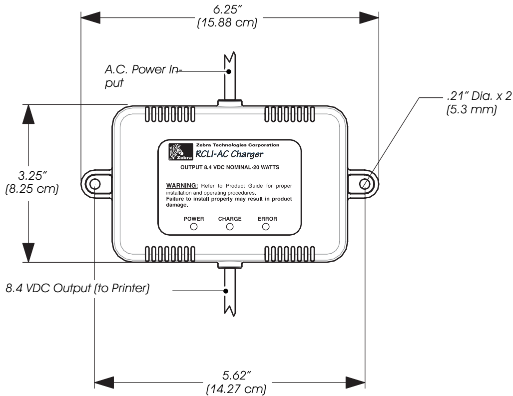
Figure 2 Charger Installation Dimensions
